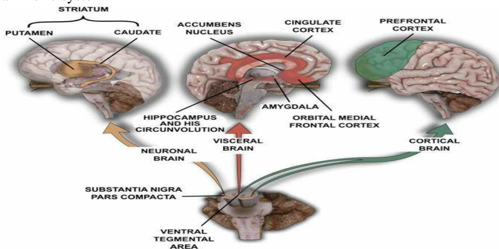
Fig. 2. Dopaminergic system
